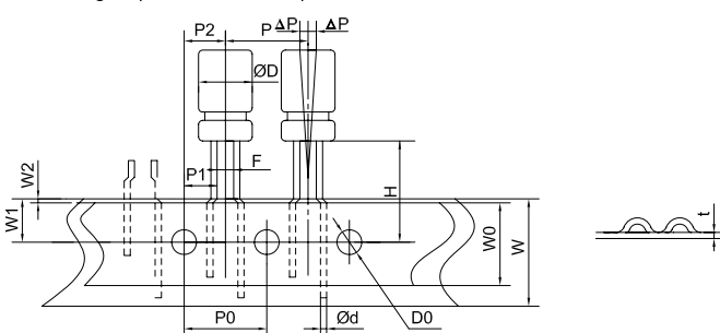
Drawing V (Ø4,Ø5,Ø6.3,Ø8)
