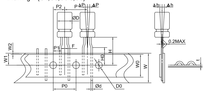
Drawing II (Ø4,Ø5,Ø6.3,Ø8)
