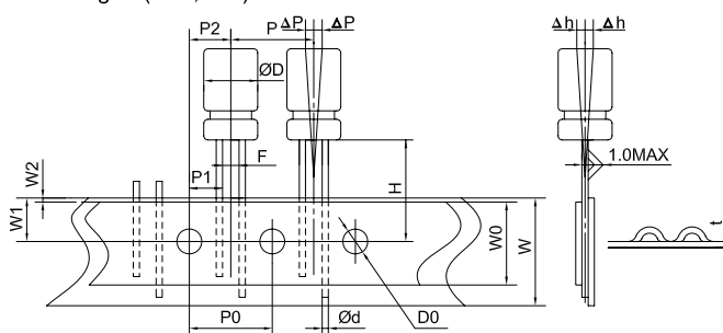
Drawing III (Ø10,Ø13)
