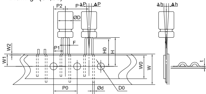
Drawing I (Ø4,Ø5)
